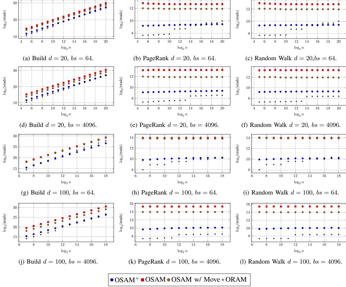
Figure 13: Read complexity results across Build, PageRank, and Random Walk for all (d, bs) configurations. Note l = 50 and df = 0.9 where applicable.
